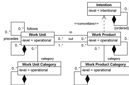
Fig. 10: The final process metamodel.
