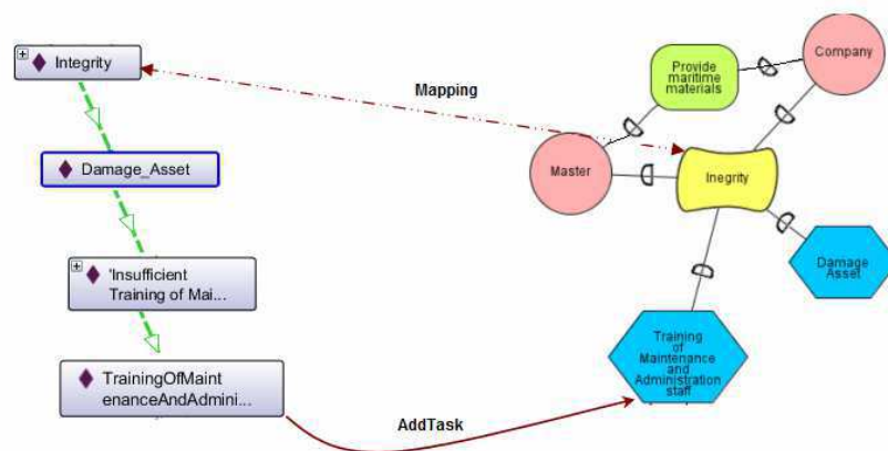
Figure 2. Example of the use of the security ontology in the analysis of security requirements
